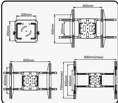
Hole Pattern
